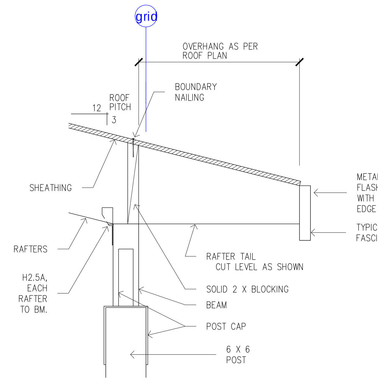
Eave at Unit #4 Entry Canopy 7
