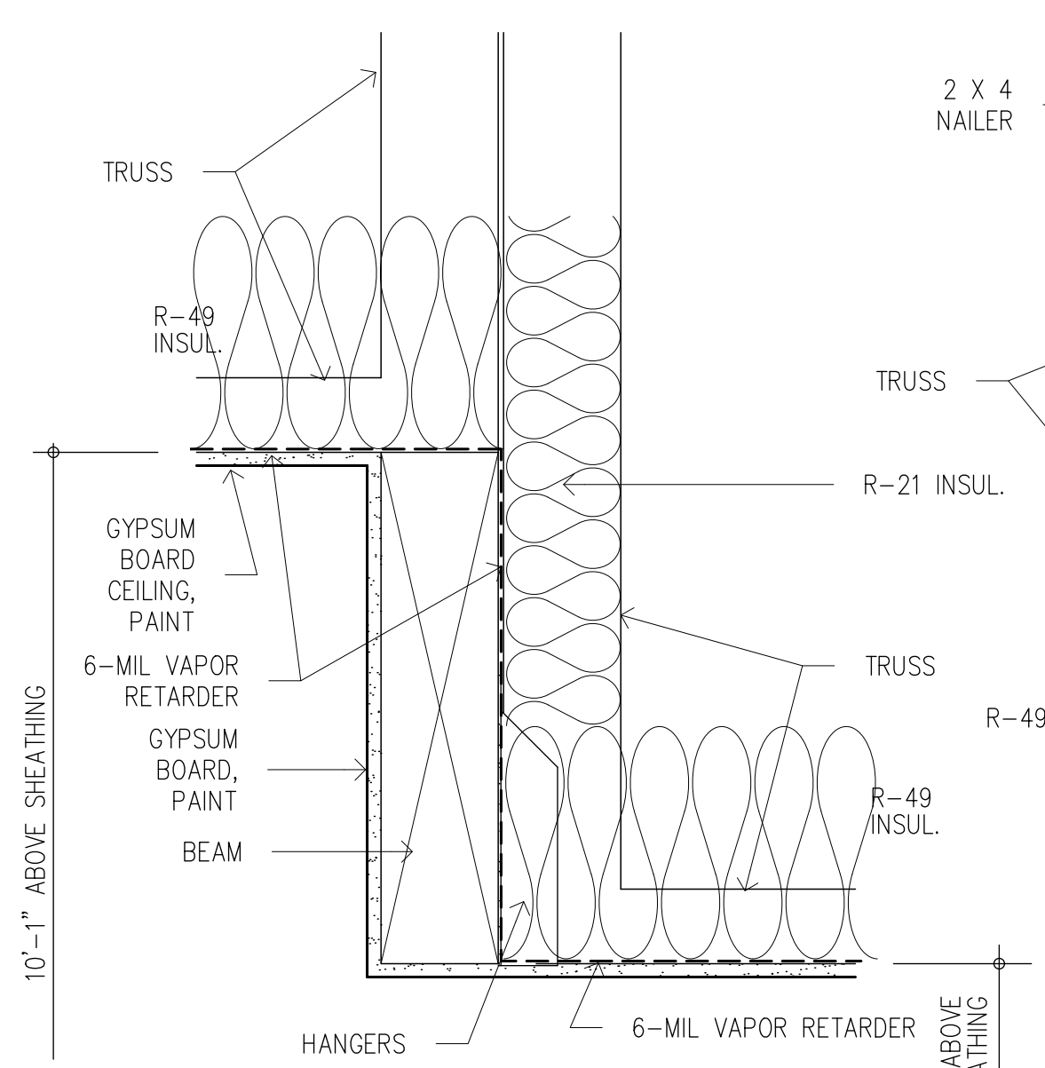
Roof Transition 2 SEE DTL. 2/S9 FOR ADDITIONAL INFORMATION
