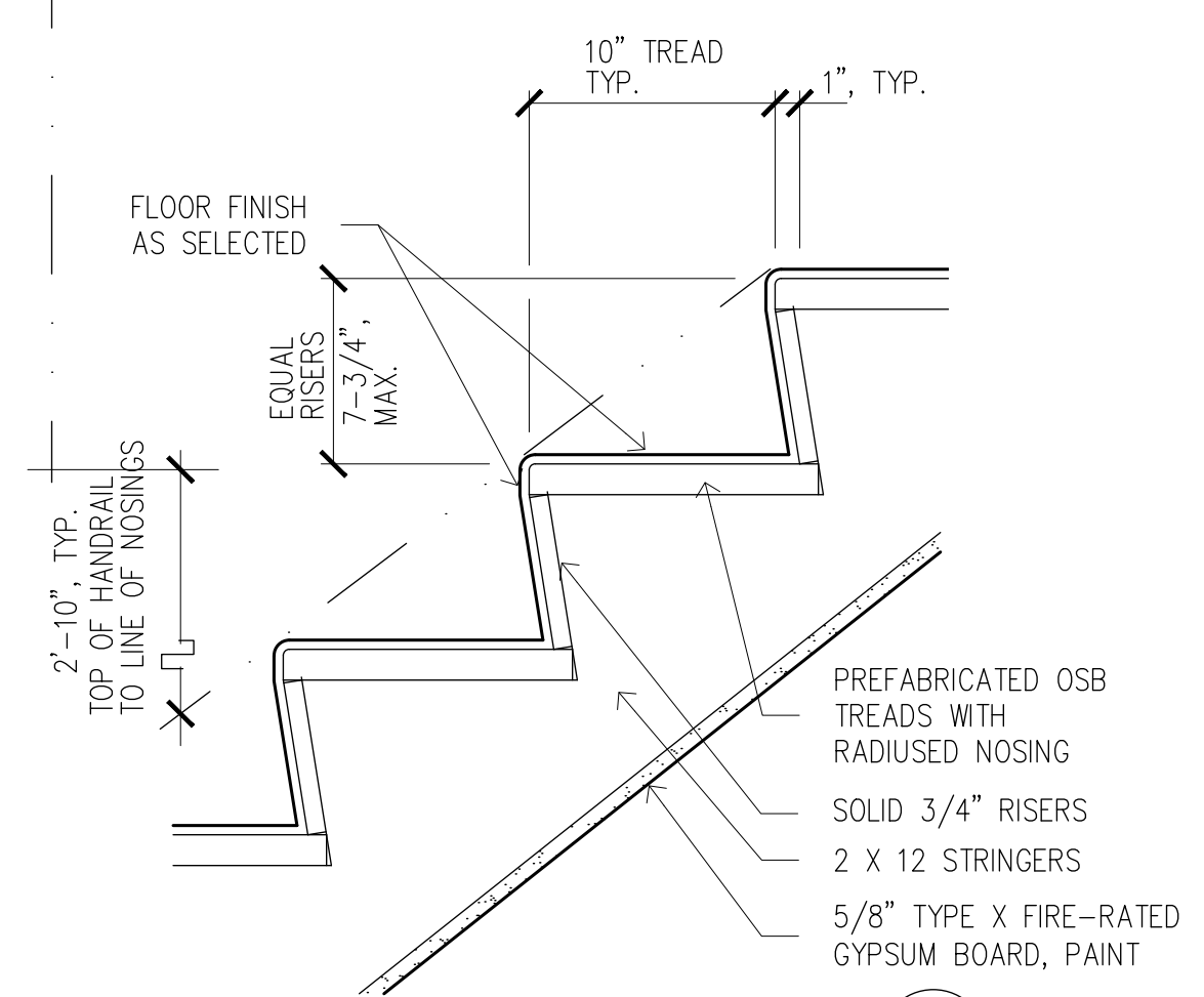
Typical stairs 7
