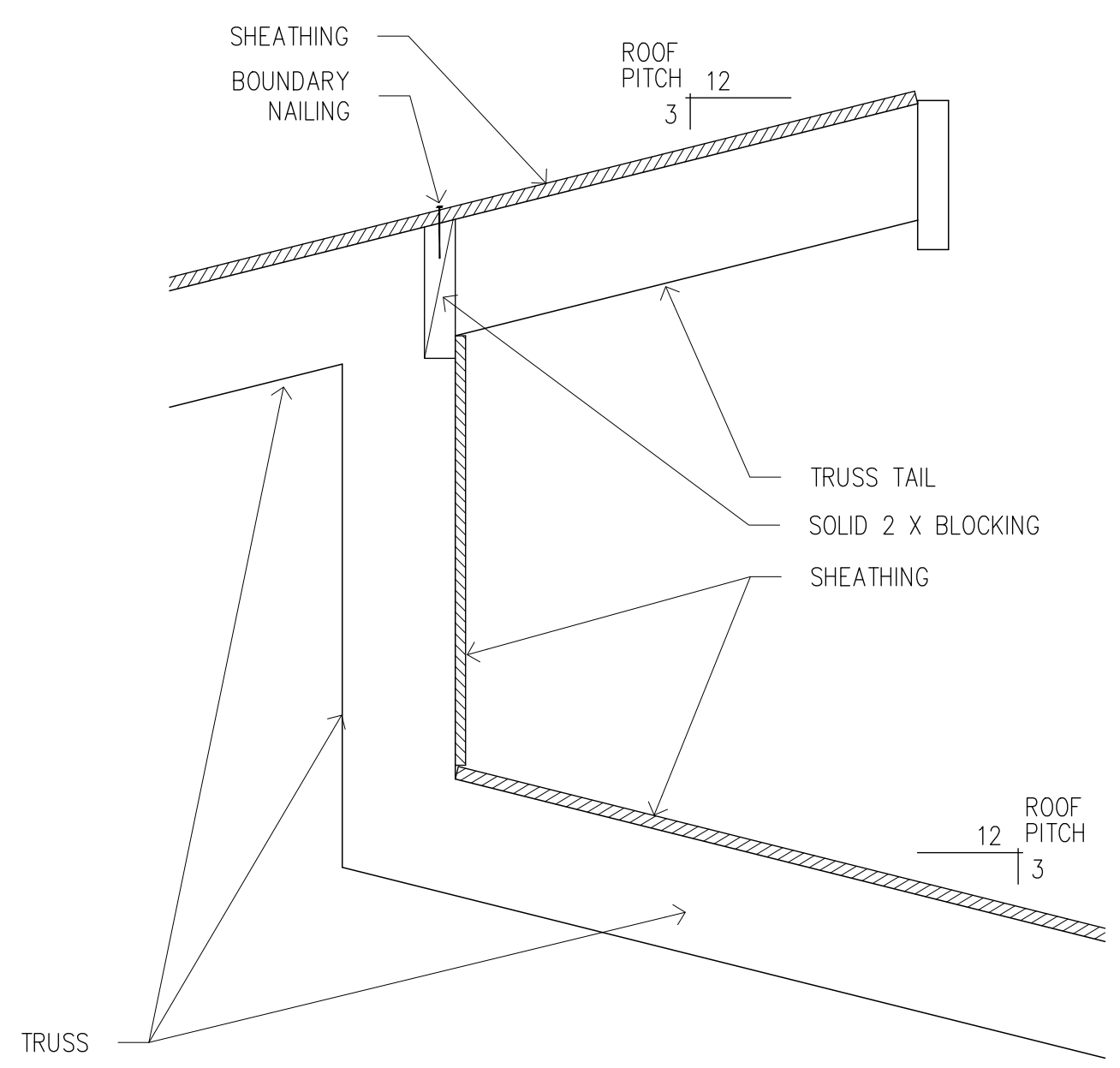
Ridge/ Headwall 11 SEE DTL. 11/A20 FOR ADDITIONAL INFORMATION
