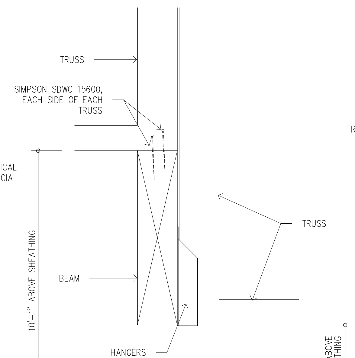
Roof Transition 2 SEE DTL. 2/A20 FOR ADDITIONAL INFORMATION
