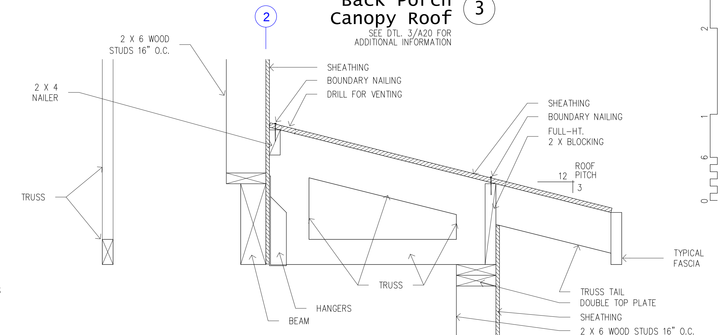
Eyebrow Truss at Bedroom Pop-Out 1 SEE DTL. 1/A20 FOR ADDITIONAL INFORMATION
