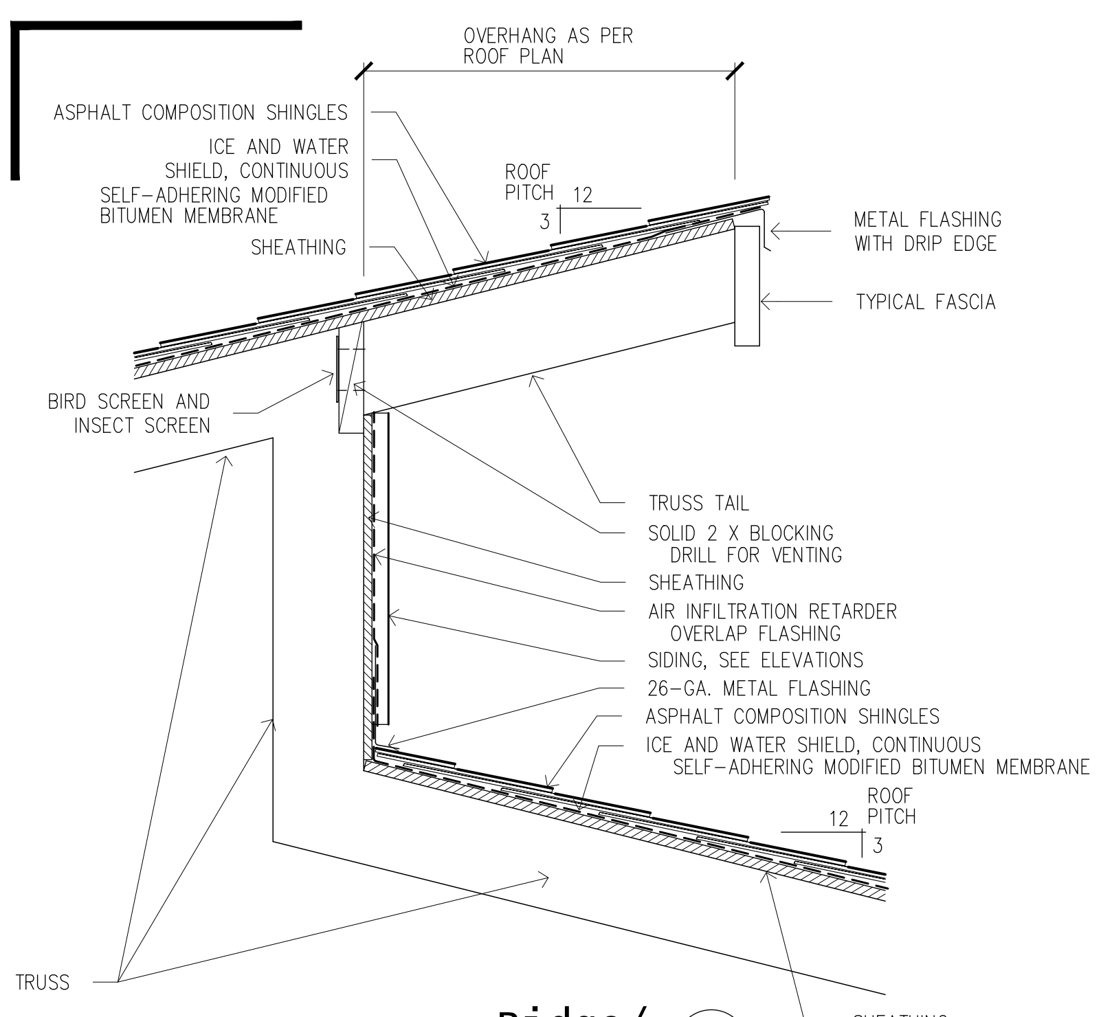
Ridge/Headwall 11 SEE DTL. 11/S9 FOR ADDITIONAL INFORMATION
