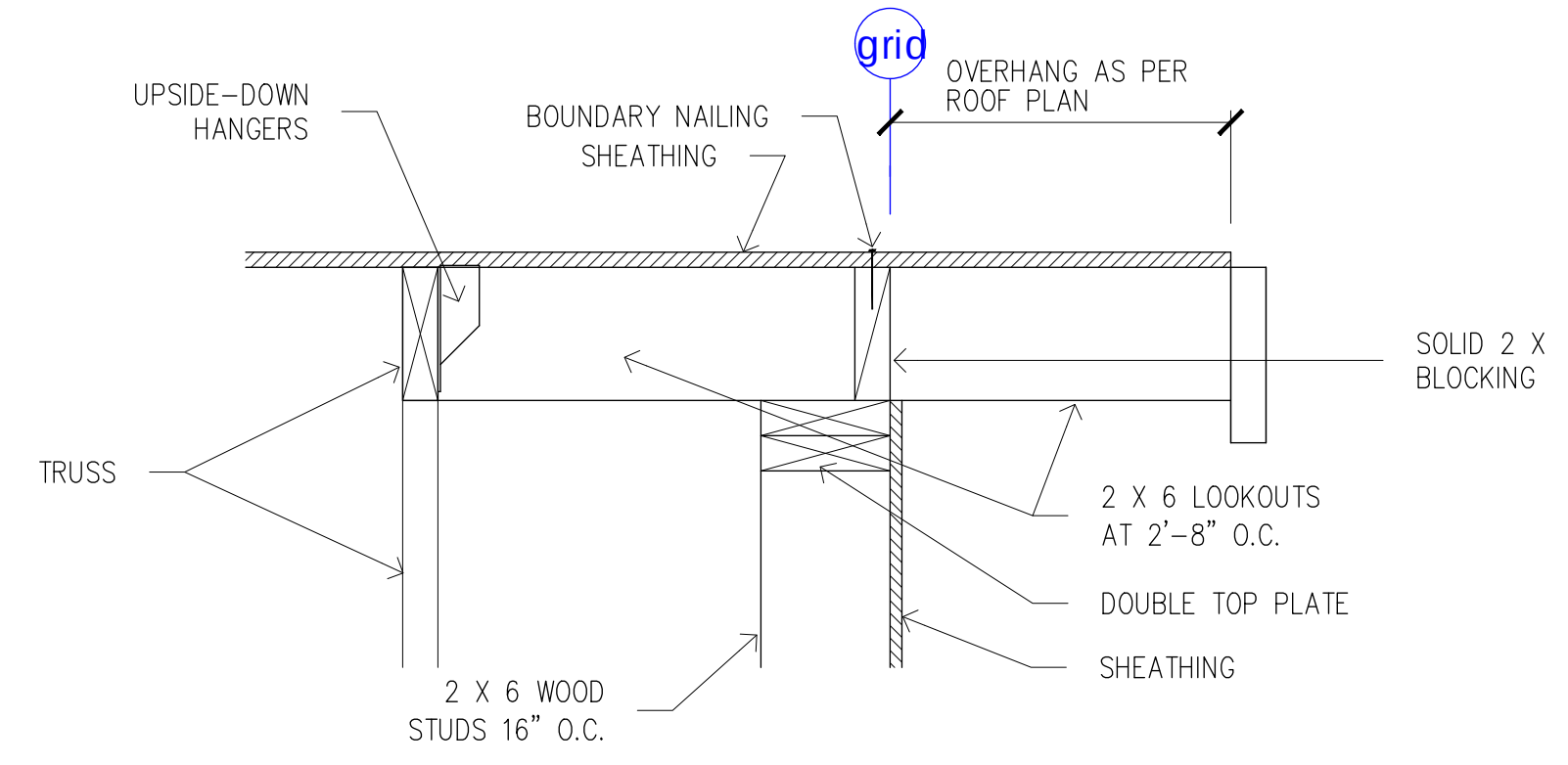
Typical Rake 10 SEE DTL. 10/A20 FOR ADDITIONAL INFORMATION
