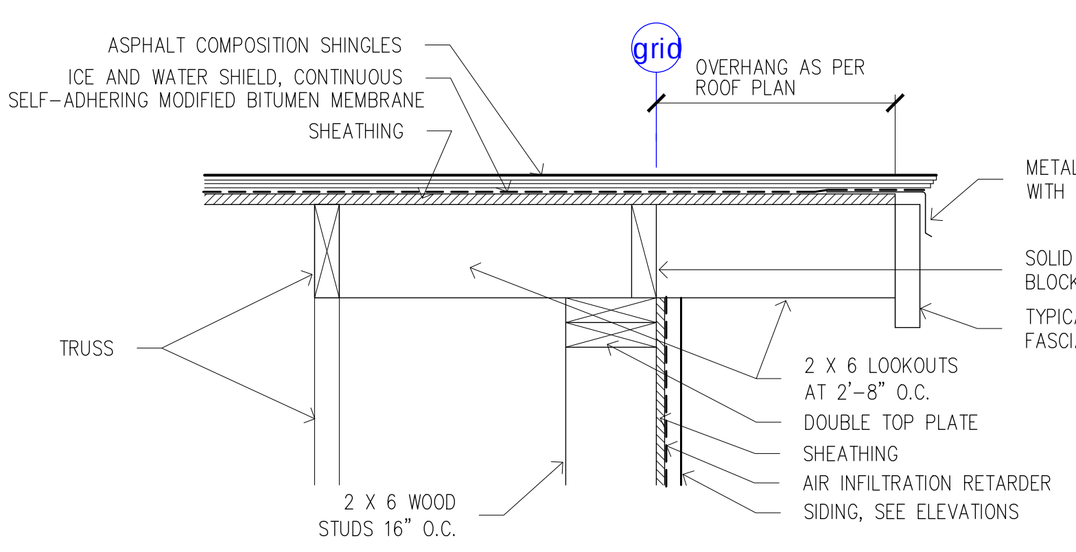
Typical Rake 10 SEE DTL. 10/S9 FOR ADDITIONAL INFORMATION
