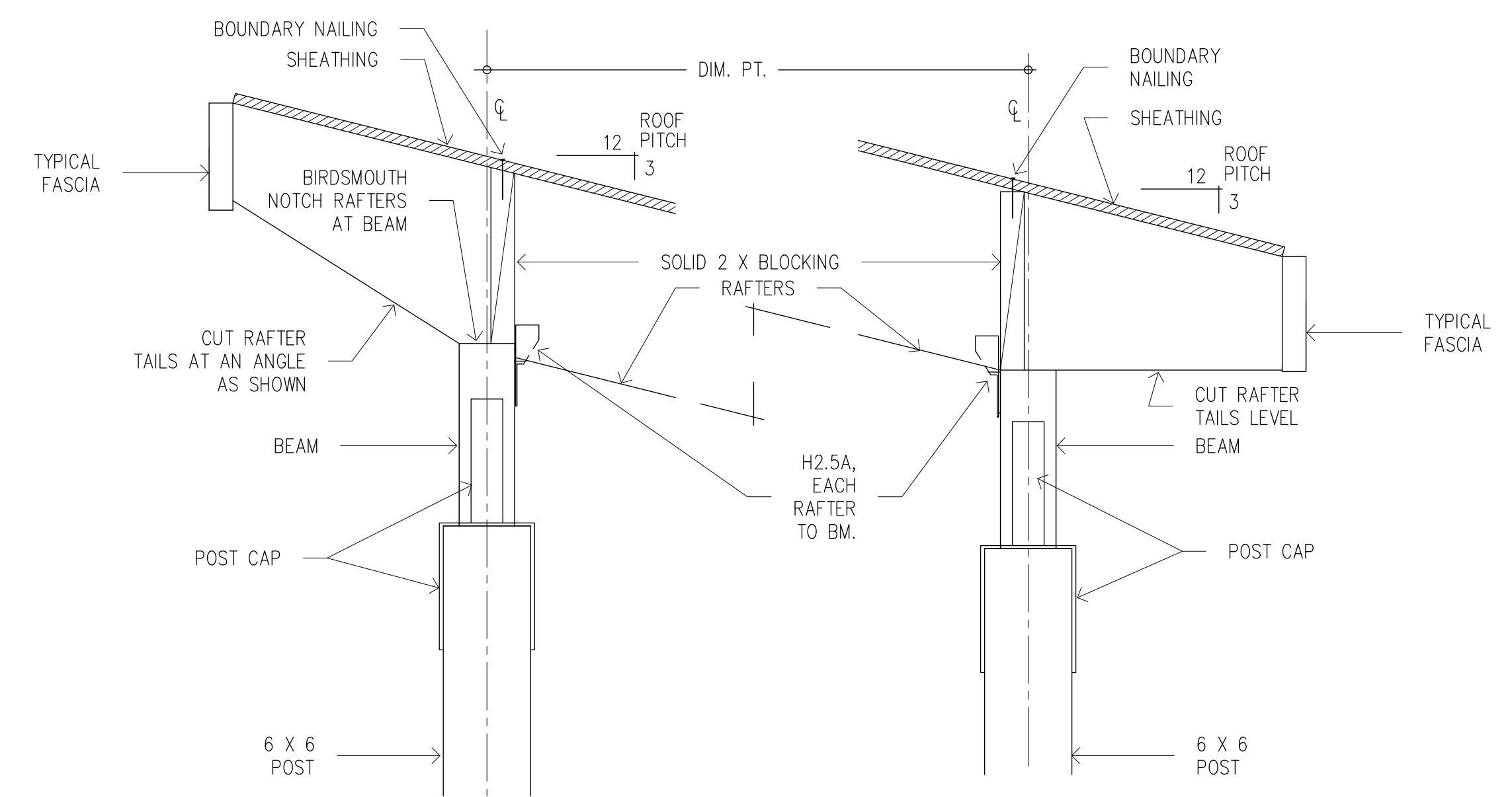
Back Porch Canopy at Unit #4 4 SEE DTL. 4/A18 FOR ADDITIONAL INFORMATION
