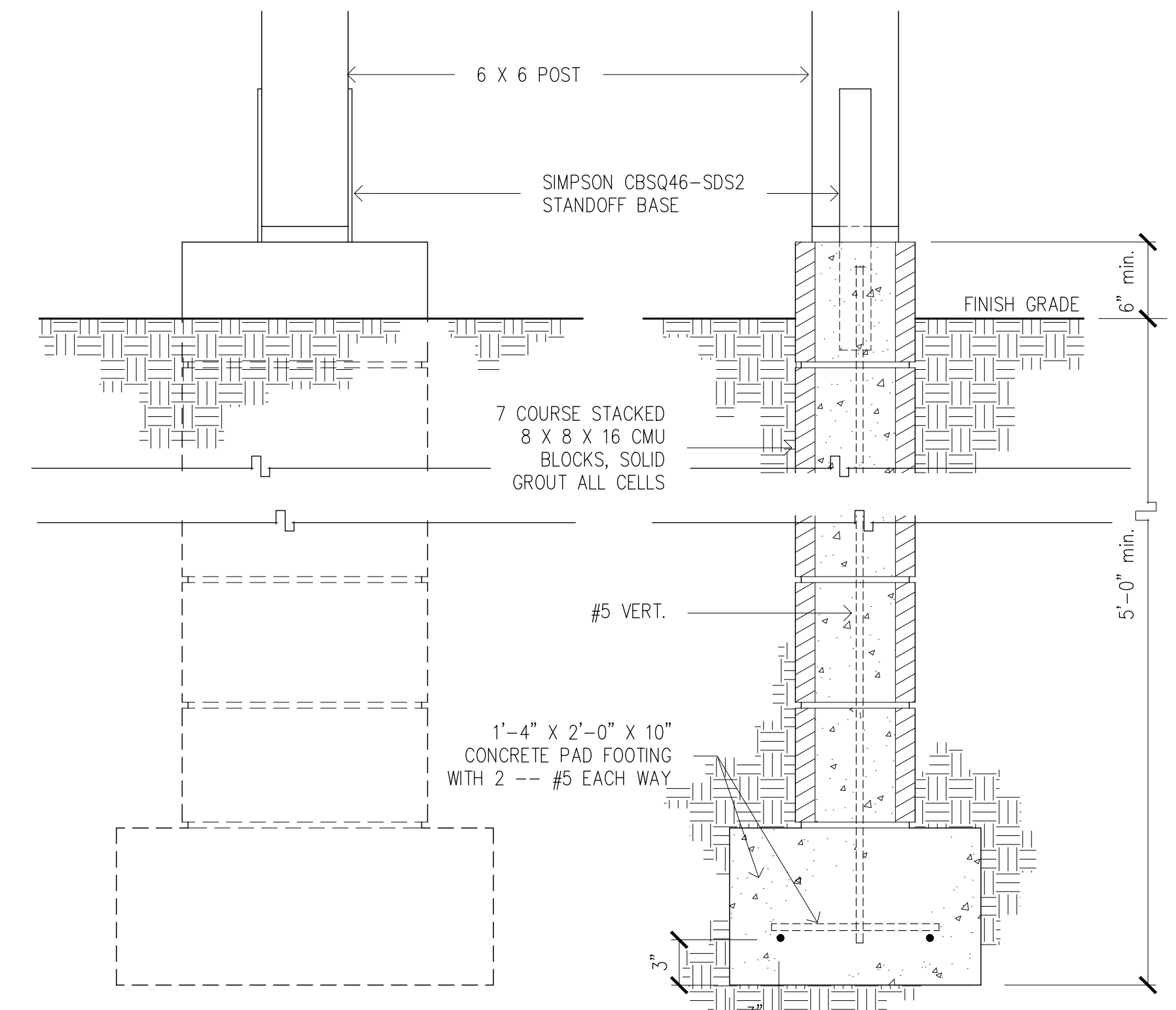
Porch Foundation 2
