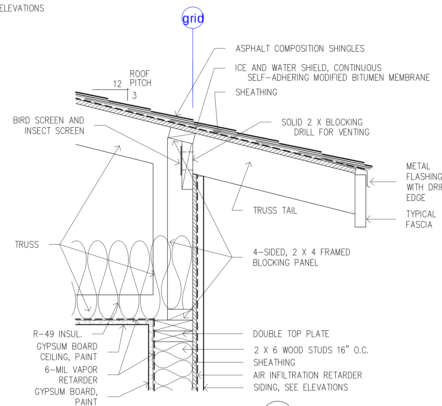
Eave 6 SEE DTL. 6/S9 FOR ADDITIONAL INFORMATION
