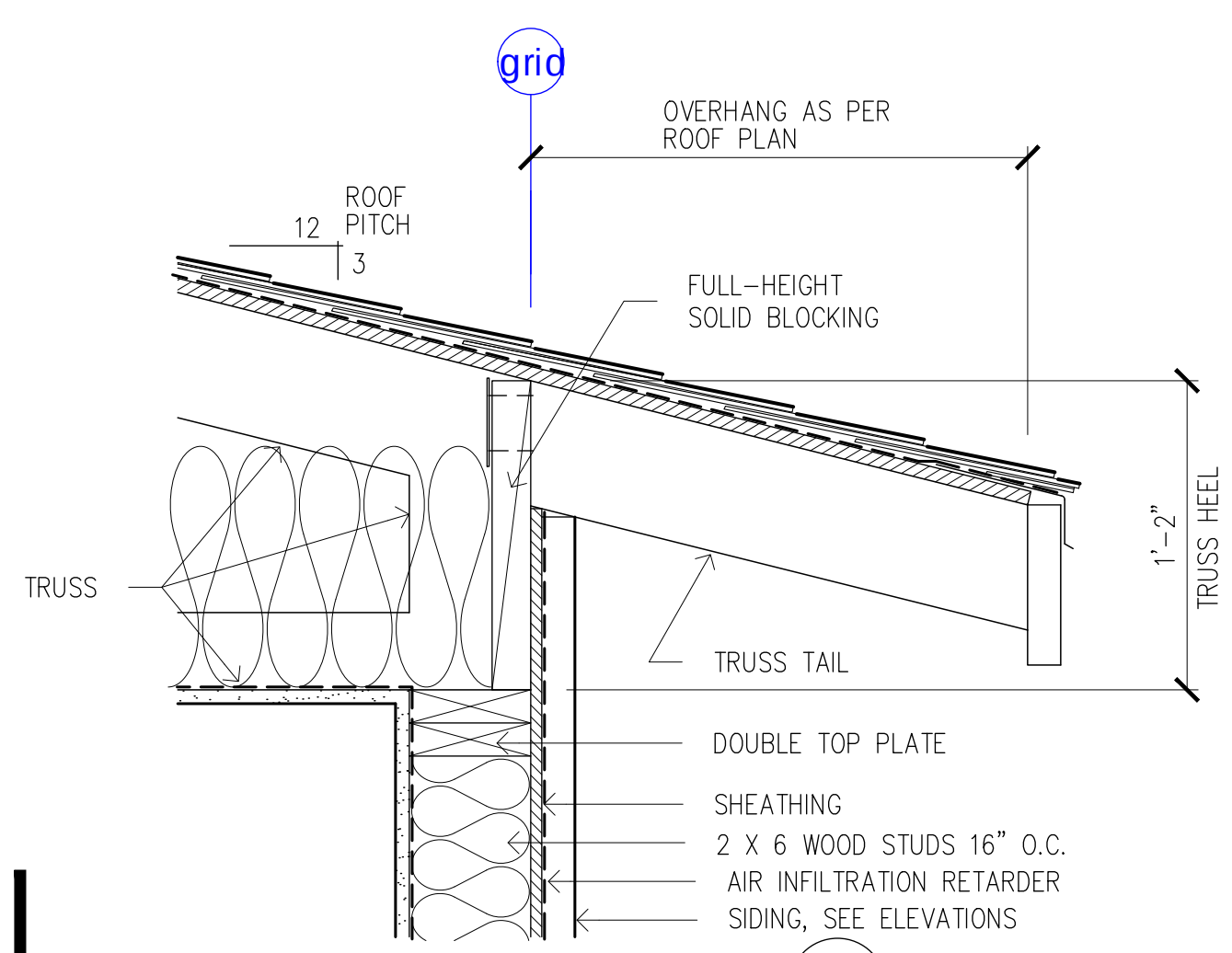
Eave 9 SEE DTL. 9/S9 FOR ADDITIONAL INFORMATION
