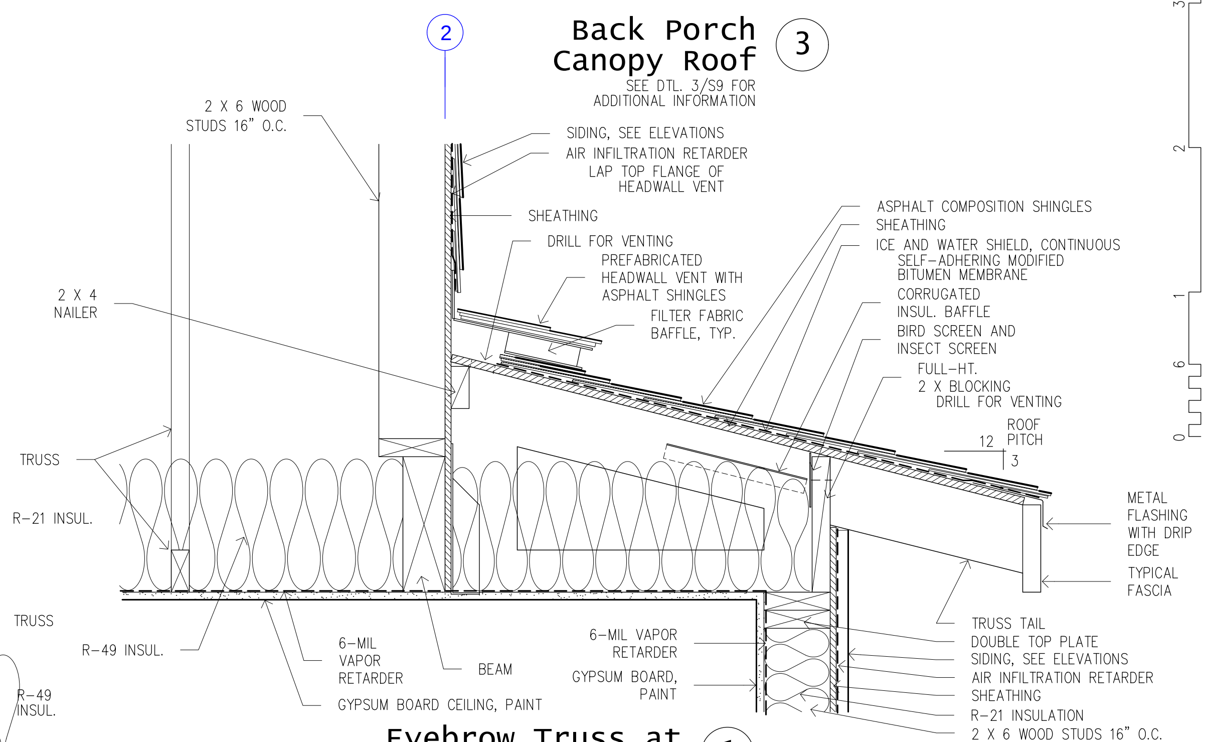
Eyebrow Truss at Bedroom Pop-out 1 SEE DTL. 1/S9 FOR ADDITIONAL INFORMATION
