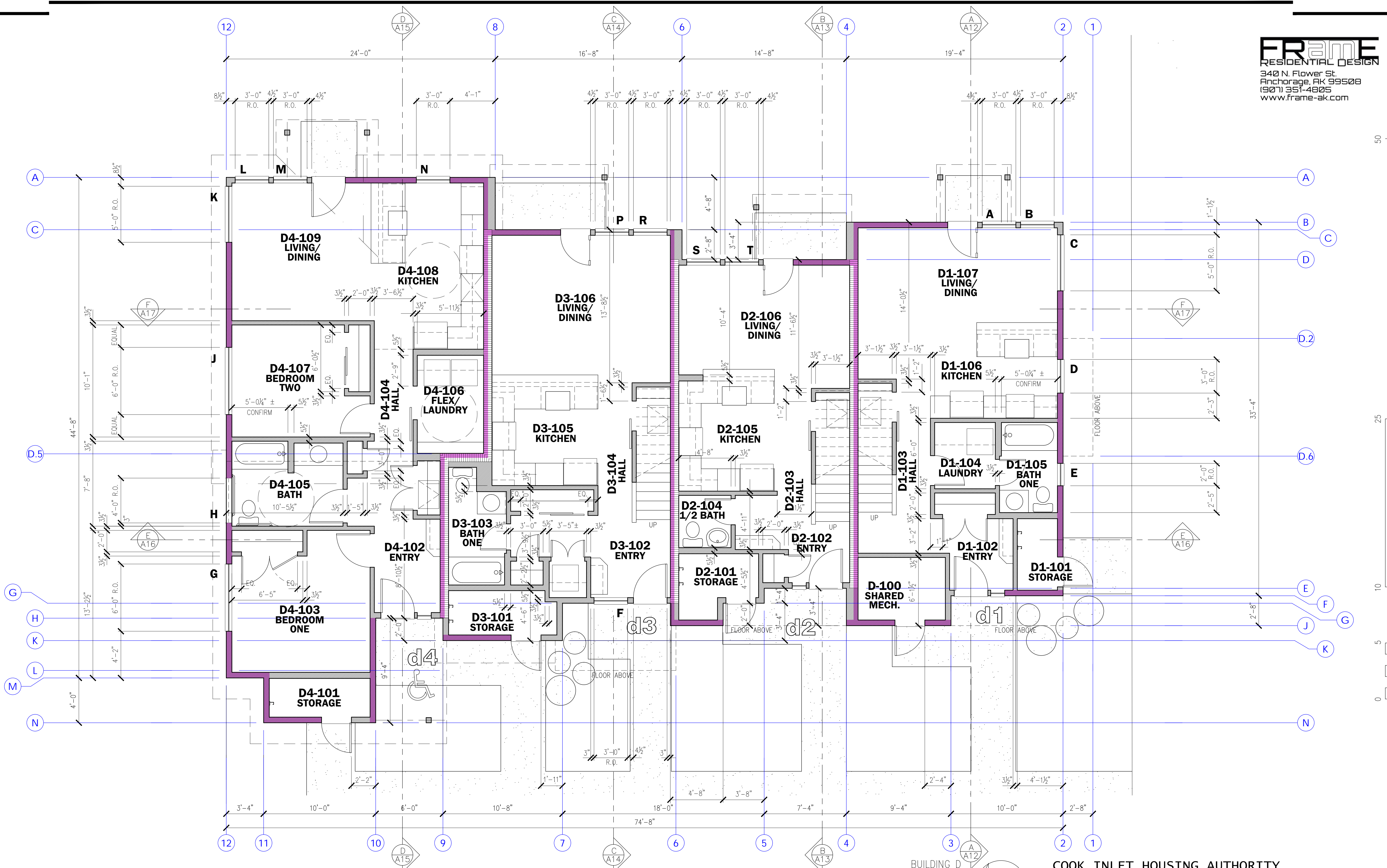
BUILDING D Overall First Floor Plan
